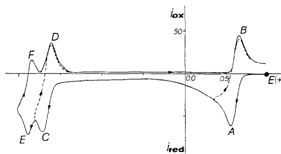
Fig. 1. Cyclic voltammetric curves recorded on a 4 \times 10^{-3} M [\text{Cu}(2,9\text{-DMP})_2](\text{NO}_3)_2 , 0.1 M tetraethylammonium tetrafluoroborate, DMF solution. Pt working electrode; 0.2 \text{ V s}^{-1} potential scan rate; room temperature. ● Starting potential for the initially cathodic scan. Potential ( E expressed in V) is referred to SCE. Current ( i ) in \mu\text{A} .
