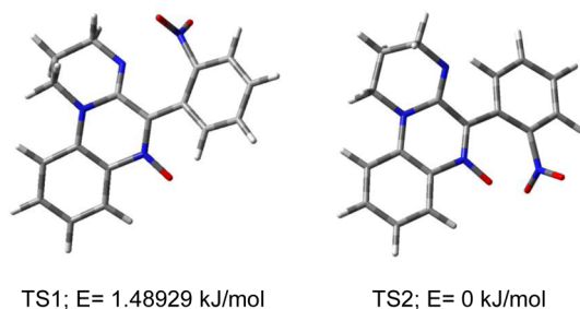
Figure 7. Transition states for the enantiomerization of compound 1b computed at the B3LYP/6-31+G(d,p) level.
