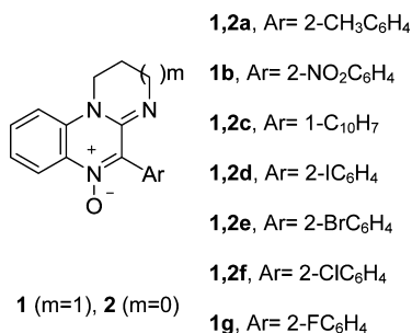
Scheme 1. General Structure of Amidinoquinoxaline N -Oxides
