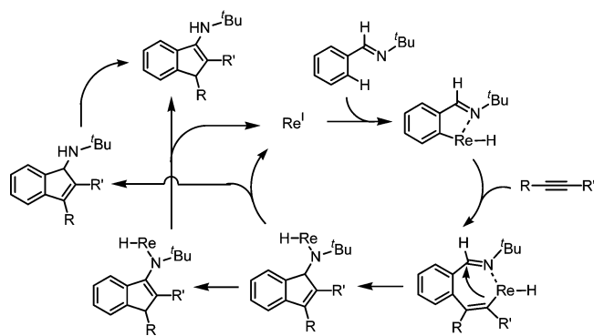
Scheme 1. Proposed Mechanism of the Formation of Indene Derivatives
