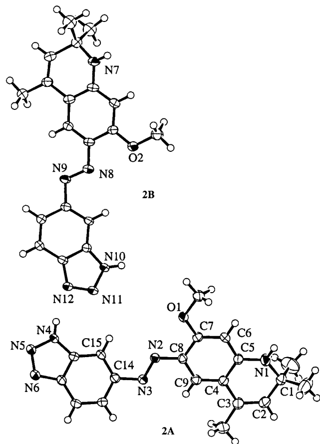
Figure 2. The molecular conformations of 2 with essential atom labels. Selected distances and angles ( \text{\AA} and ^\circ ): N(4)-N(5) 1.341(3) N(5)-N(6) 1.308(4) N(1)-C(1) 1.443(4) C(1)-C(2) 1.484(5) C(3)-C(4) 1.470(4) C(4)-C(5) 1.419(4) N(3)-N(2)-C(8) 115.1(2) N(2)-N(3)-C(14) 112.8(2) C(1)-C(2)-C(3) 125.3(3) N(3)-N(2)-C(8)-C(7) -167.7(3) N(2)-N(3)-C(14)-C(15) 26.4(4).
