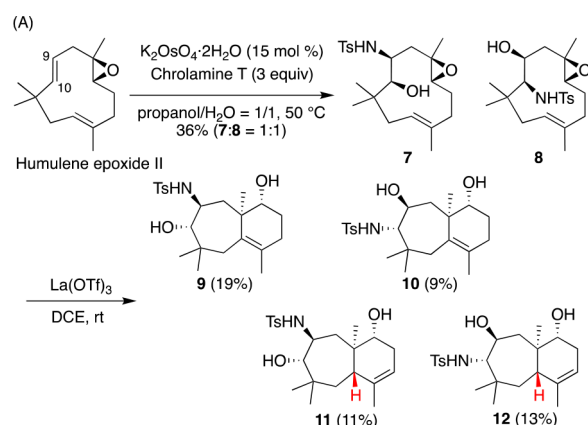
Figure 2. (A) Synthesis of unnatural terpenoid-like compounds 9 – 12 .
