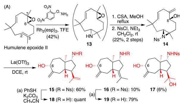
Figure 3. (A) Synthesis of salivalane-type compounds 15 – 17 .
