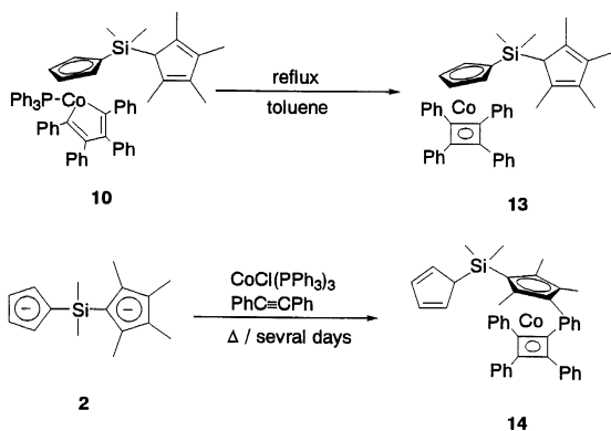
Scheme 8.
