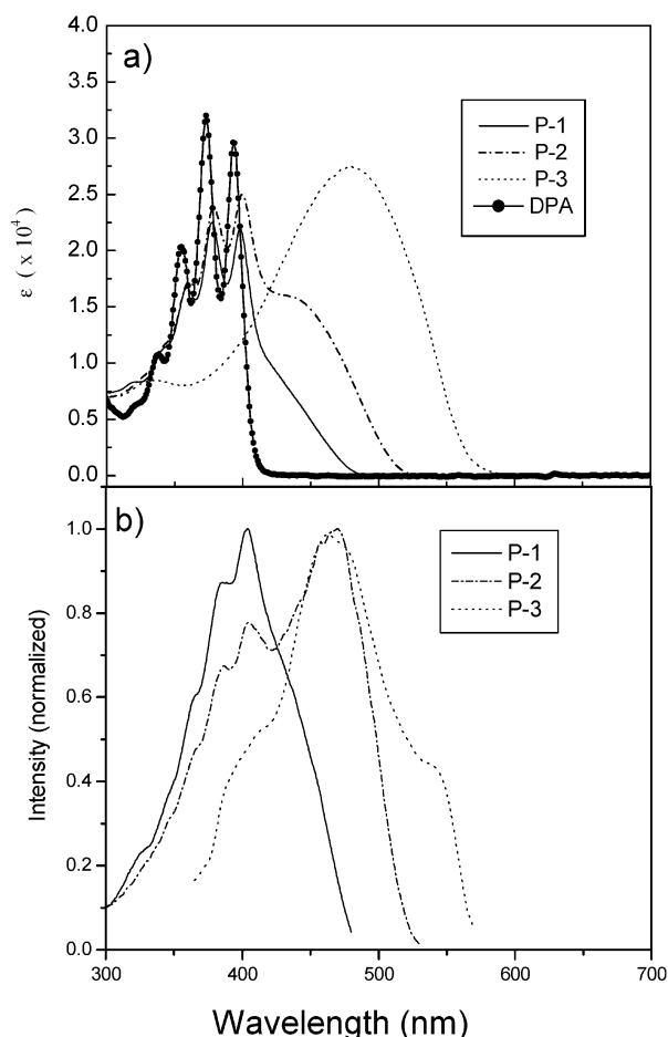
Figure 2. a) Absorption spectra of P-1 , P-2 , P-3 , and 9,10-diphenylanthracene ( DPA ); b) one-photon excitation spectra of P-1 , P-2 , and P-3 (fluorescence monitored at 500 nm, 550 nm, and 600 nm for P-1 , P-2 , and P-3 , respectively) in 1,1,2,2-tetrachloroethane. Concentration = 10^{-4} mol/L in repeating unit.
