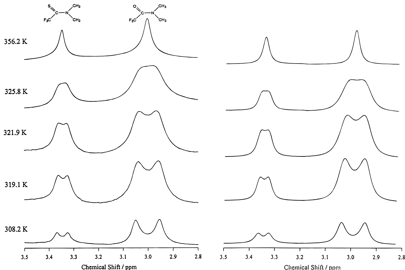
Figure 2. (a) Experimental (left) and (b) calculated (right) temperature-dependent gas-phase 300-MHz ^1\text{H} NMR spectra of the N -methyl protons in N,N -dimethylthiotrifluoroacetamide and N,N -dimethyltrifluoroacetamide.
