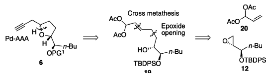
Scheme 4. Revised Strategy To Access the trans -THF 6
