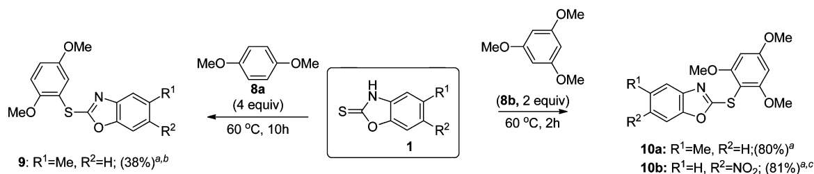
Scheme 2. Reaction of Thione with Trimethoxybenzene and Dimethoxybenzene
