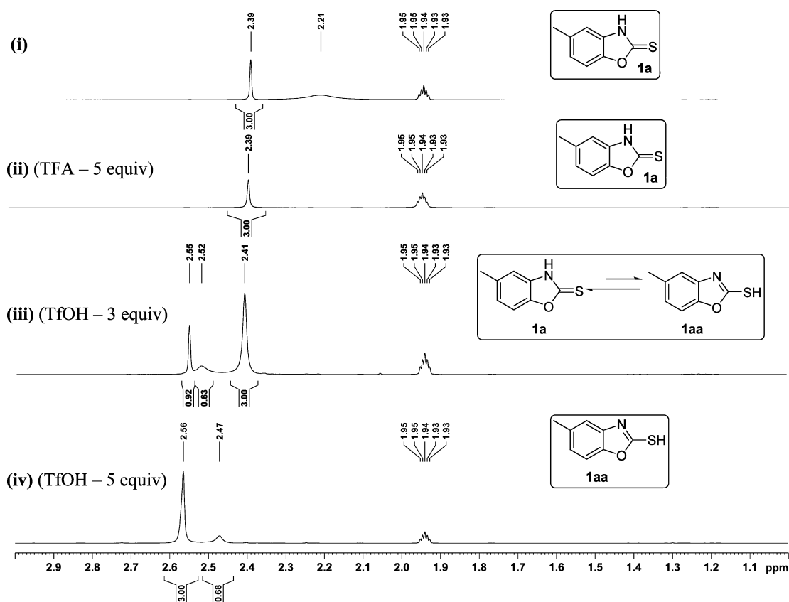
Figure 3. ^1\text{H} NMR experiments: (i) 1a (4.5 mg) in \text{CD}_3\text{CN} (0.5 mL); (ii) 1a (1 equiv) in TFA (5 equiv) and \text{CD}_3\text{CN} (0.45 mL); (iii) 1a (41.25 mg) in TfOH (3 equiv) and \text{CD}_3\text{CN} (0.94 mL); (iv) 1a (20.5 mg) in TfOH (5 equiv) and \text{CD}_3\text{CN} (0.45 mL).
