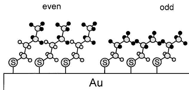
Figure 2. Idealized structure for n -alkanethiols with an odd (right) number of carbons and even (left) number of carbons. The odd alkyl chain length positions the terminal C–C bond more parallel to the plane of the surface compared to the even alkyl chain length. The parallel orientation places the terminal hydrogen atoms in a more favorable position to react with impinging ion beam while hindering access to the terminal carbon.
