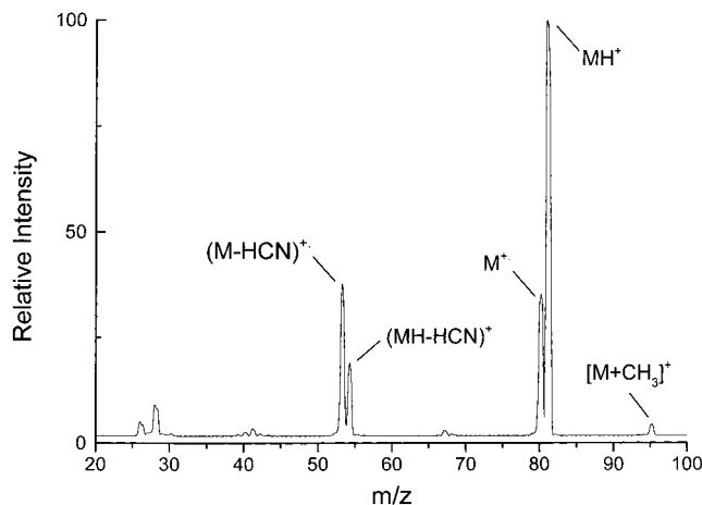
Figure 3. The 20 eV collision of pyrazine ion M^{+} ( m/z 80) with a CH_3(CH_2)_{17}-S-Au SAM film. The base peak in the spectrum MH^{+} ( m/z 81) represents a reaction of the probe ion and a hydrogen atom from the SAM film. The peak at m/z 95 is the formal addition of methyl to the M^{+} ion. The two most abundant fragment ions at m/z 53 and 54 represent [M - HCN]^{+} and [MH - HCN]^{+} .
