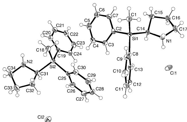
Figure 3. ORTEP plot of the molecular structure of ( S )-2-(methyl-diphenylsilyl)pyrrolidine-HCl [( S )-5-HCl]. [14] Displacement ellipsoids drawn at the 50% probability level.
