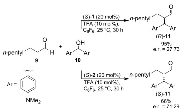
Scheme 4. Organocatalytic asymmetric \alpha -alkylation of n -octanal ( 9 ) with bis[4-(dimethylamino)phenyl]methanol ( 10 ).
