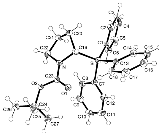
Figure 4. ORTEP plot of the molecular structure of ( S )-2-(triphenylsilyl)- N -boc-pyrrolidine [( S )- 7 ]. [14] Displacement ellipsoids drawn at the 50% probability level.
