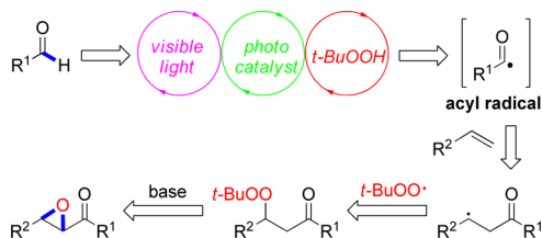
Scheme 1. Visible-Light-Promoted Photoredox Preparations of \alpha,\beta -Epoxy Ketones from Styrenes and Benzaldehydes under Alkaline Conditions
