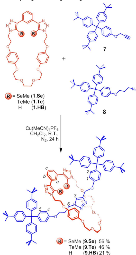
Scheme 3. Synthesis of Chalcogen Bonding Rotaxanes and their Hydrogen Bonding Analogue
