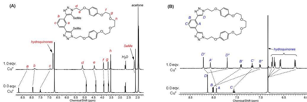
Figure 1. Partial ^1\text{H} NMR spectra showing macrocycles (A) 1.Se in d_6 -acetone and (B) 1.HB in \text{CD}_2\text{Cl}_2 in the presence of 0.0 and 1.0 equivalents of \text{Cu}(\text{CH}_3\text{CN})_4\text{PF}_6 (500 MHz, T = 298 K).
