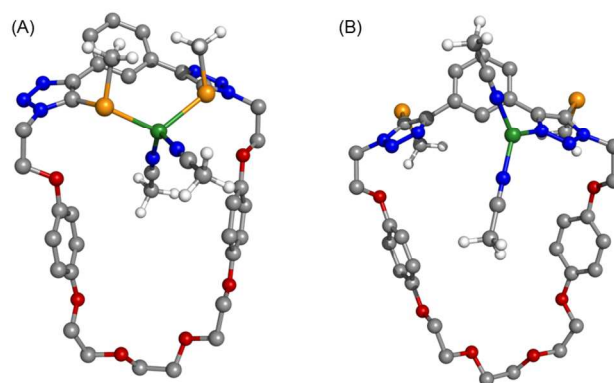
Figure 2. DFT optimized structures of the possible coordination modes of [\text{Cu1.Se}(\text{CH}_3\text{CN})_2]^+ complex using (A) model A and (B) model B.
