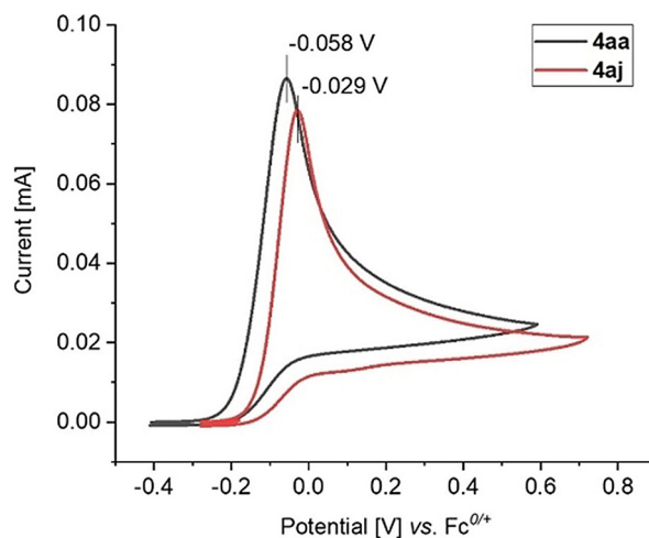
Figure 2. Cyclic voltammetry studies. Conditions: 4aa (2.5 mM) or 4aj (2.5 mM), n\text{Bu}_4\text{NPF}_6 (0.1 M), MeCN, 100 \text{ mVs}^{-1} .
