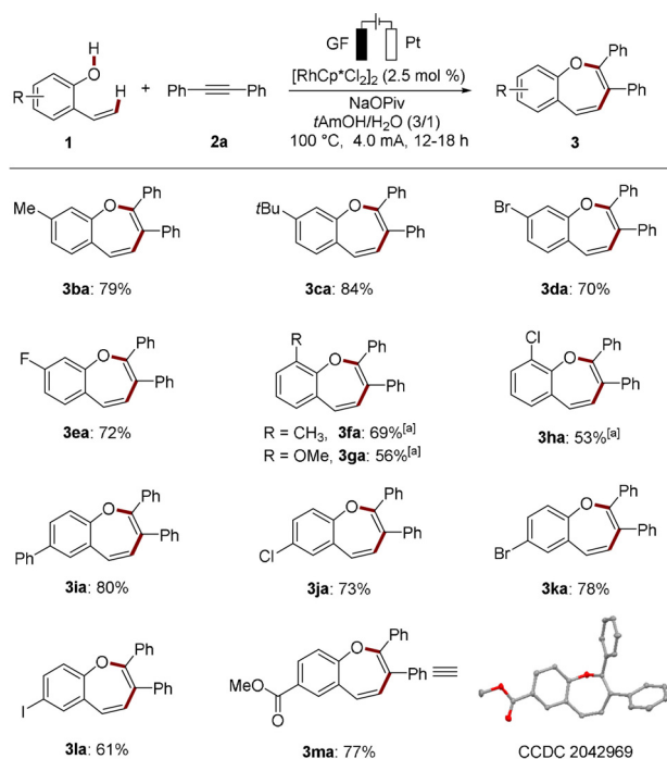
Scheme 3. Rhodaelectro-catalyzed [5+2] cycloadditions with 2-vinylphenols. [a] 5.0 mol % [RhCp*Cl 2 ] 2 .
