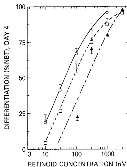
Figure 2. Dose-response curves for retinoids in the HL-60 differentiation assay: (○) trans -retinoic acid; (□) 1a , (▲) 1c . Differentiation is measured as the percentage of cells that reduce NBT after a 4-day incubation in the presence of the retinoid. This value for control cells was 4%. The values presented are from at least three independent experiments with duplicate measurements. Bars, SD. The two blocks gave reproducible values so close so as to preclude any bar representations.
