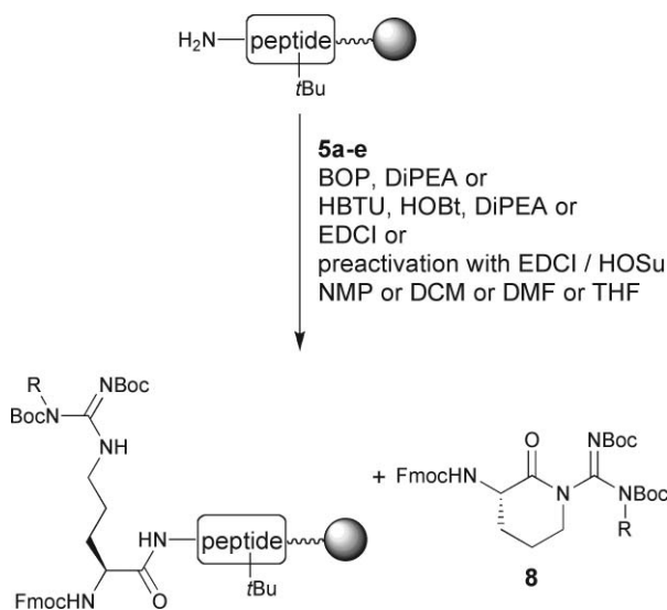
Scheme 2 Side product formation.
