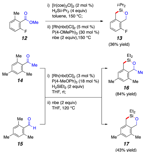
Scheme 4. Sequential, Exhaustive, Reductive Benzylic C_{sp^3} -H Silylation of Aromatic Esters, Ketones, and Aldehydes
