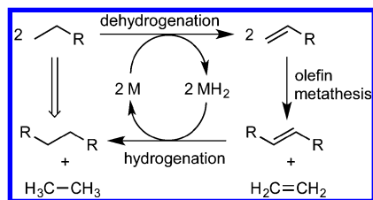
Figure 1. Alkane metathesis via tandem dehydrogenation–hydrogenation and olefin metathesis catalysis.
