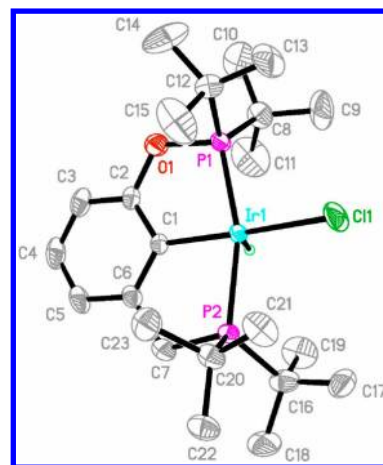
Figure 4. Thermal ellipsoid plot of (t\text{Bu}^4\text{PCOP})\text{IrHCl} ( 2c ). Hydrogen atoms other than the hydride ligand omitted for clarity.
