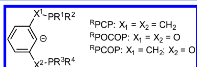
Figure 2. Pincer ligands of the type used in this work ( X = \text{CH}_2 or \text{O} ; R = \text{alkyl} ).
