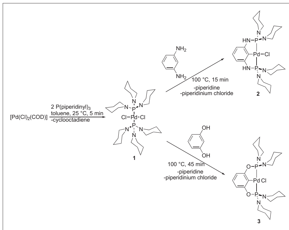
Scheme 1. Synthesis of the catalysts 2 and 3 .
