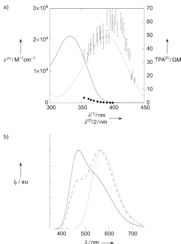
Figure 2. Photophysical properties of 4-PYMPO at 293 K. a) One-photon absorption (molar absorption coefficient, \epsilon , versus \lambda ; pH 2=---, pH 14=—) and two-photon absorptivity (TPA versus \lambda/2 ; pH 2=○, pH 14=●) spectra. b) Normalized steady-state fluorescence emission ( I_F ) after one-photon excitation at \lambda_{\text{exc}}=356 nm (pH 2=---, pH 6=---, pH 14=—). Solvent: Britton–Robinson buffer [53] (0.1 M).
