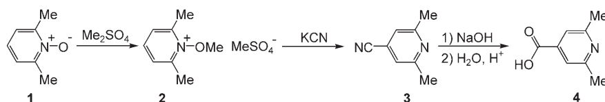
Scheme 2. Synthesis of the 2,6-dimethylisonicotinic acid precursor ( 4 ) used to make 4-PYMPOM.
