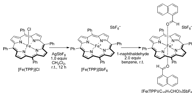
Scheme 1. Synthesis of the [\text{Fe}(\text{TPP})(\text{C}_{10}\text{H}_7\text{CHO})_2]\text{SbF}_6 Complex
