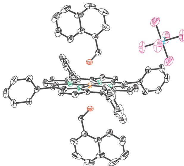
Figure 1. ORTEP drawing of [\text{Fe}(\text{TPP})(\text{C}_{10}\text{H}_7\text{CHO})_2]\text{SbF}_6 .
