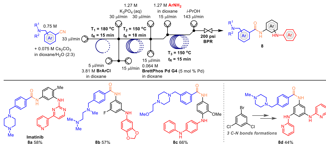
Scheme 5. Continuous Flow Synthesis of Imatinib and Analogues a
