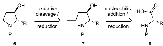
Scheme 1. Four-step synthesis of 3-hydroxy-pyrrolidines from amino acids.
