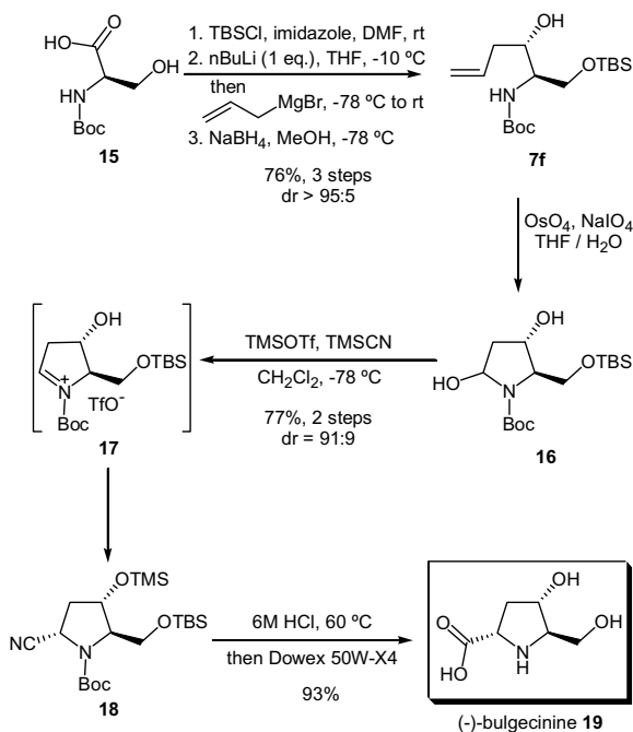
Scheme 3. Six-step asymmetric synthesis of (-)-bulgecinine from D-serine.
