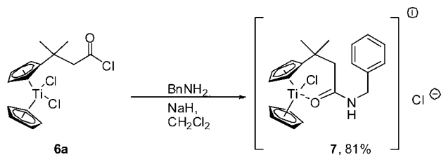
Scheme 4. Optimized Preparation of 7 by Acylation of Benzylamine with 6a
