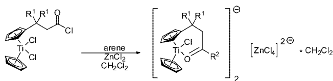
Scheme 6. Conditions for the Friedel–Crafts Acylation of 6
