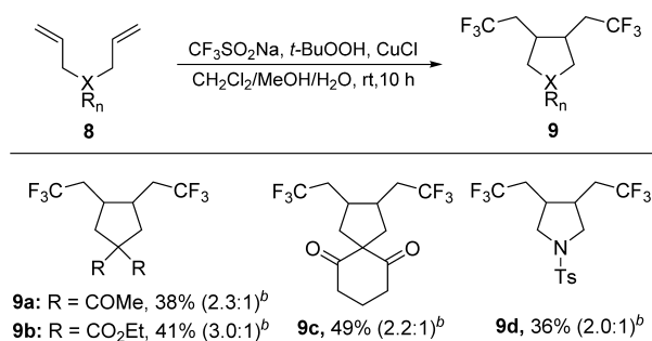
Scheme 6. Preparation of 1,4-Bis(trifluoromethylated) Products 9 a
