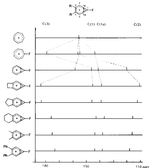
Fig. 2. ^{13}\text{C} -NMR shifts of 1-fluorocyclopropabenzene cations 3 and related compounds (see also Table 4, Exper. Part )
