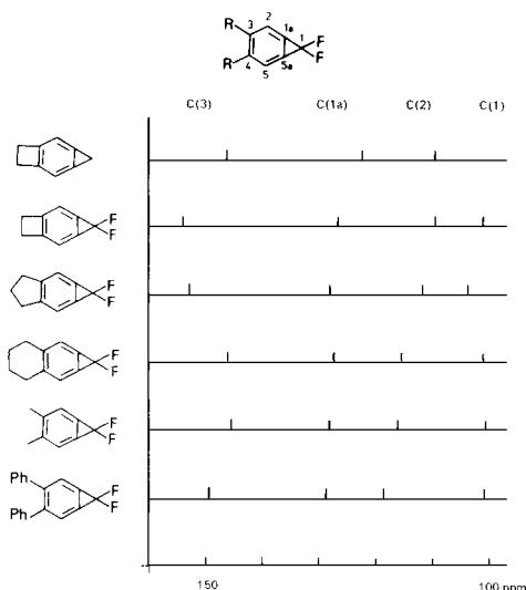
Fig. 1. ^{13}\text{C} -NMR shifts of 1,1-difluorocyclopropabenzene derivatives 4 (see also Table 3, Exper. Part )
