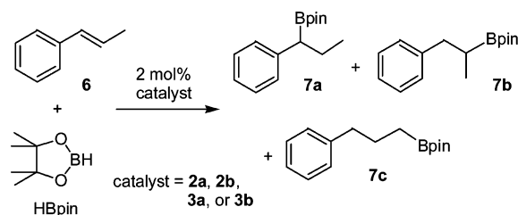
Scheme 3. Metal-Catalyzed Hydroboration of 1-Phenylpropene (6) using HBpin
