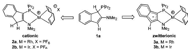
Scheme 1. Cationic and Zwitterionic \kappa^2 - P,N Rh(I) and Ir(I) Complexes Derived from 1a
