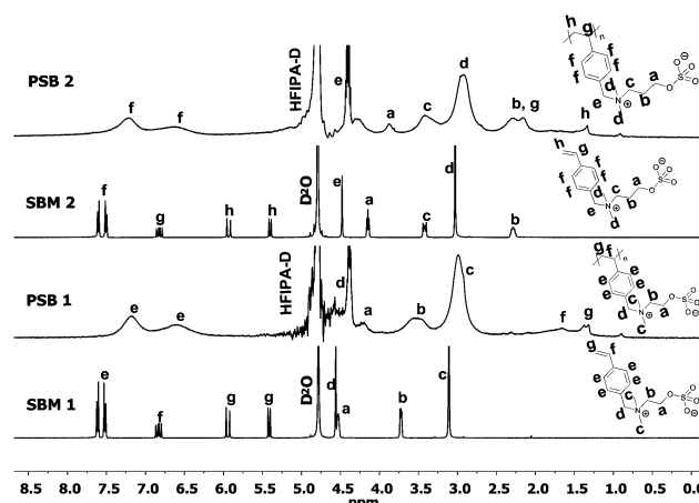
Fig. 2 1 H-NMR spectra of sulfobetaine monomers (SBM) in D 2 O and corresponding polysulfobetaines (PSB) in (CF 3 ) 2 CD 3 -OD.
