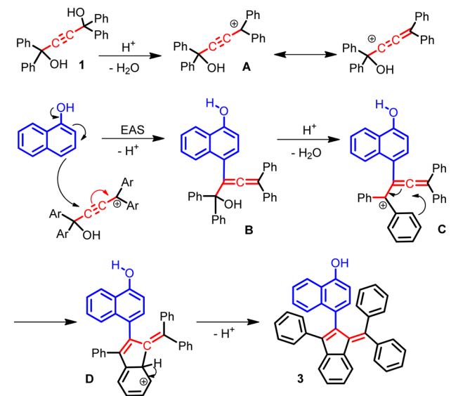
Scheme 5. Proposed Mechanism for the Formation of 1 H -Indene Dye 3 from Tetraphenylbut-2-yne-1,4-diol 1 and 1-Naphthol
