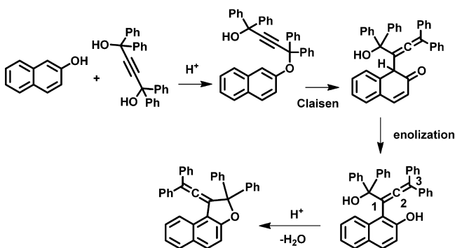
Scheme 3. Synthesis of 1,1,4,4-Tetraarylbut-2-yn-1,4-diols 1 (Ar = Ph) and 2 (Ar = p -MeOPh)
