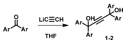
Scheme 3. Synthesis of 1,1,4,4-Tetraarylbut-2-yn-1,4-diols 1 (Ar = Ph) and 2 (Ar = p -MeOPh)
