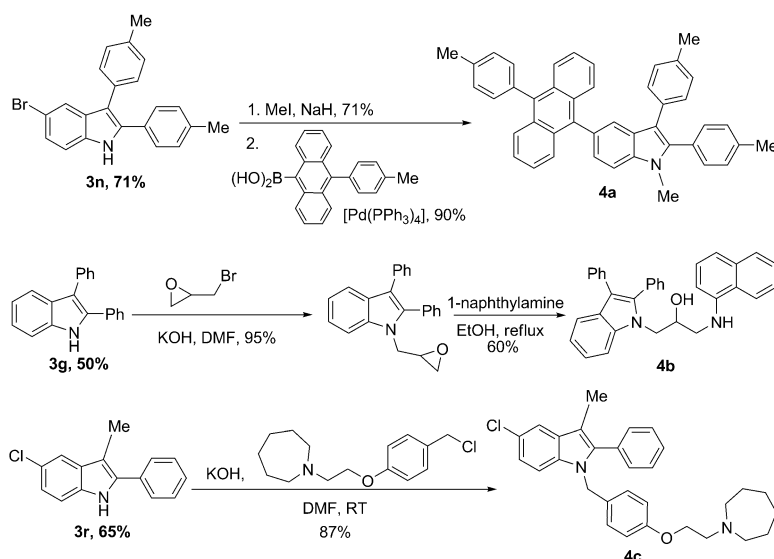
Scheme 4. Demonstration of product utilities.
