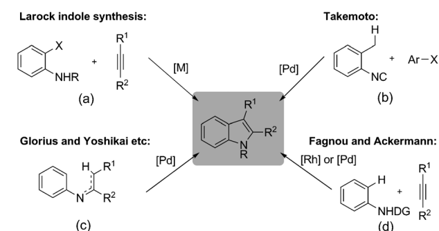
Scheme 1. Transition-metal-catalyzed indole synthesis. DG = directing group.
