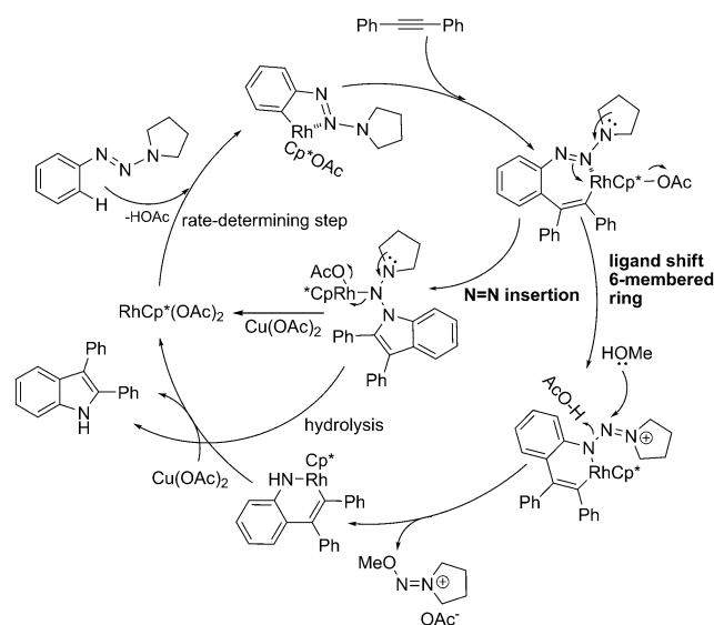
Scheme 6. Proposed mechanism of the triazene-directed NH indole synthesis.
