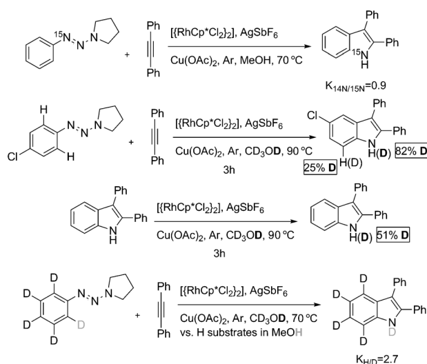
Scheme 5. Reactions using isotope-labeled substrates.
