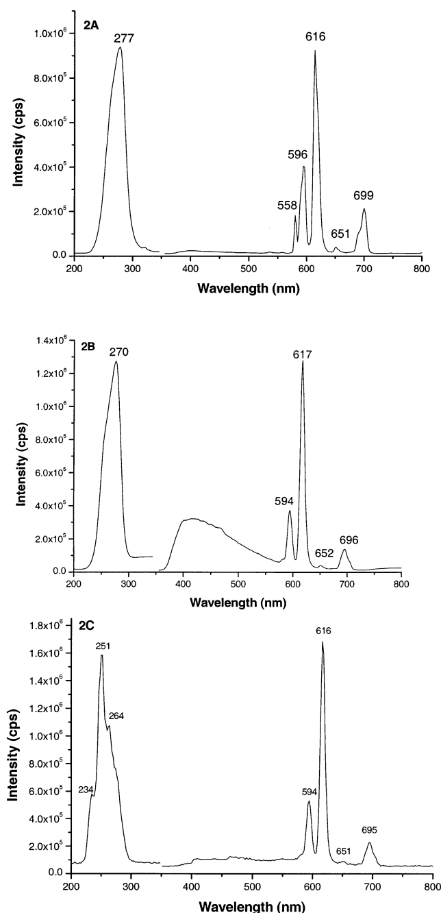
FIGURE 2. Excitation and steady-state emission spectra of the lipid 11· \text{Eu}^{3+} complex (A); the polymerized liposomes incorporating this complex (B) and time-resolved excitation and emission spectra of the polymerized liposomes (C). Solvents were methanol and HEPES buffer (25 mM, pH 7.0) for the lipid and the liposome, respectively. All spectra are blank subtracted. Spectra were recorded with the following parameters: (A) excitation band-pass = 4 nm, emission band-pass = 4 nm, cut-off filter at 350 nm; (B) excitation band-pass = 8 nm, emission band-pass = 6 nm, cut-off filter at 350 nm; (C) excitation band-pass = 16 nm, emission band-pass = 12 nm, cut-off filter at 350 nm, delay time = 30 \mu\text{s} , gate time = 9 ns, 100 pulses per data point. All excitation spectra were recorded at the maximum emission wavelength; all emission spectra were recorded at the maximum excitation wavelength.
