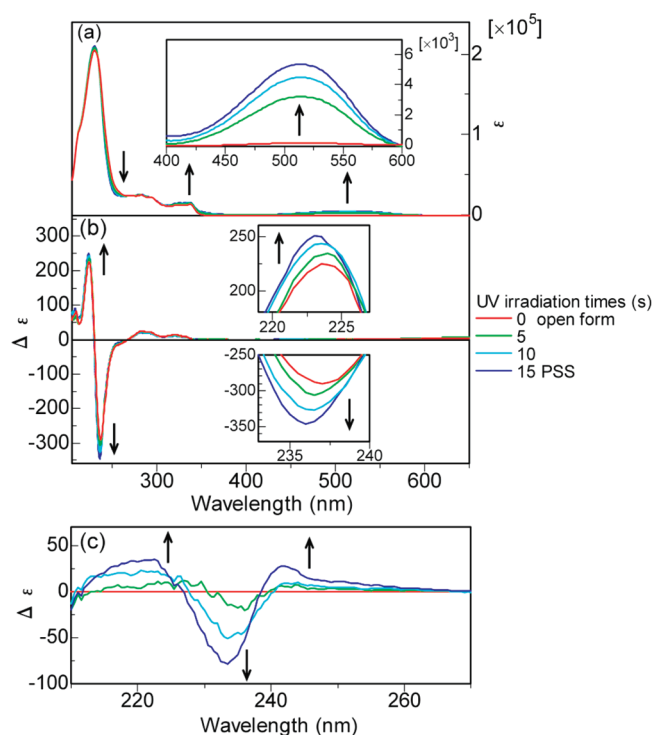
Figure 2. (a) Changes in UV–vis absorption and (b) CD spectra of (R)-D1 in n -heptane ( 1.5 \times 10^{-5} M) upon irradiation with UV light ( \lambda = 254 nm, 16 W) for 0, 5, 10, and 15 s at 30 °C. Inset shows the expanded spectra. (c) Difference spectra given by subtraction of the CD spectrum of (R)-D1 (open form) from those of (R)-D1 (PSS) upon irradiation with UV light for 0, 5, 10, and 15 s.
