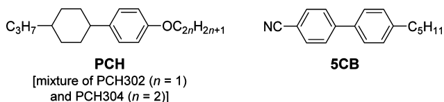
Scheme 3. Structures of Nematic Liquid Crystals
