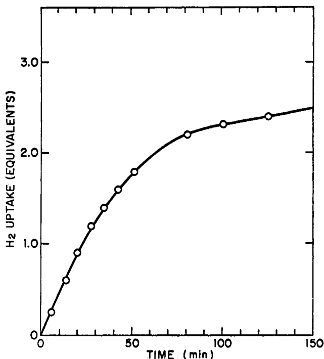
Figure 1. Catalytic reduction of 3-methylbicyclo[1.1.0]butanecarbonitrile.
