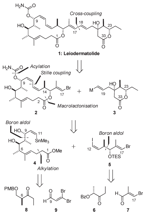
Scheme 1. Retrosynthetic Analysis of Leiodermatolide
