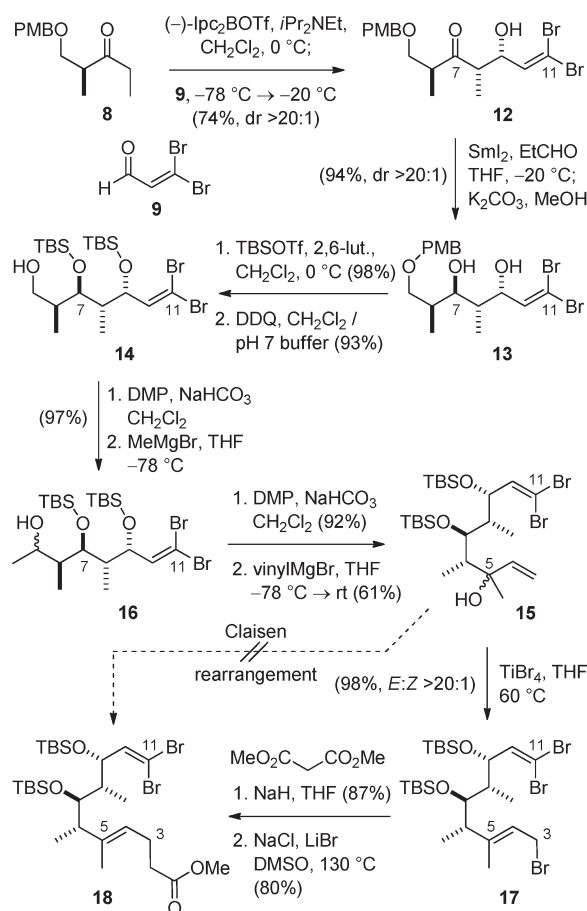
Scheme 3. Preparation of C1–C11 Fragment 18
