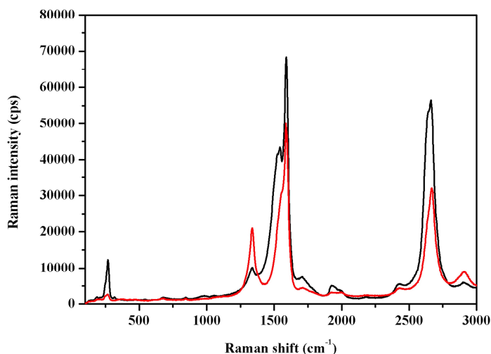
Figure 3. Raman spectra of pristine SWNTs (black) and NHS-PFPA-functionalized SWNTs prepared using microwave-assisted reaction conditions (red).
