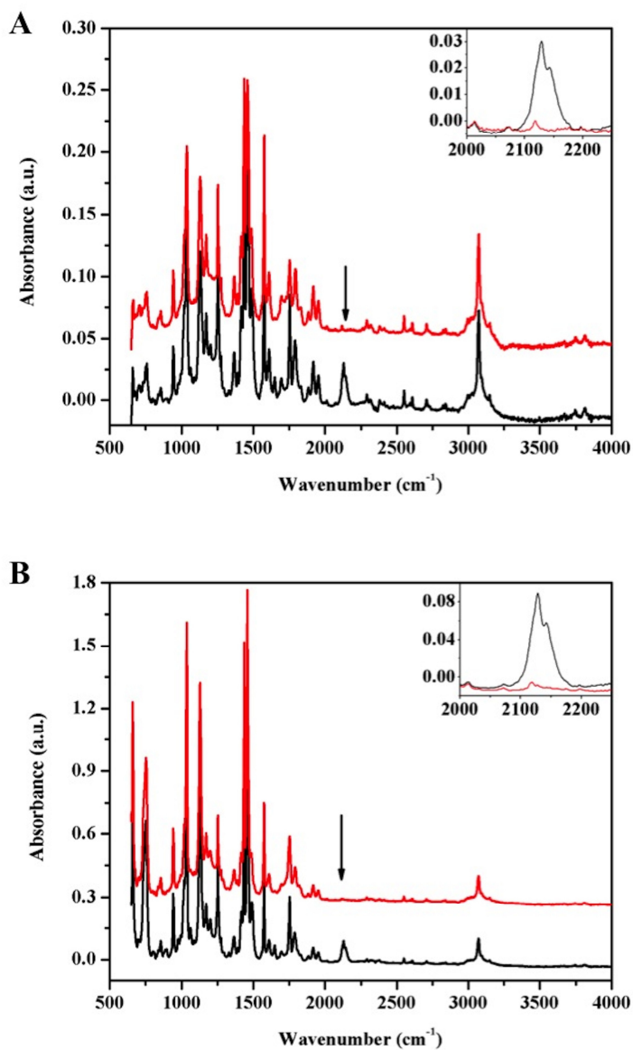
Figure 2. IR spectra of the reaction of PFPA-NHS with SWNTs under (A) conventional oil bath heating at 130 °C for 3 days, and (B) microwave radiation at 150 °C for 1 h before (black) and after (red) reactions. The arrows indicate the azide absorption, which are enlarged in the insets.
