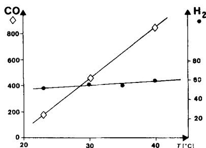
Fig. 6. Efficiency of CO and \text{H}_2 photogeneration as a function of temperature. Conditions of Exper. 18, Table 2, at saturation with \text{CO}_2 and irradiating with a 1000-W Xe lamps for 16 h.
