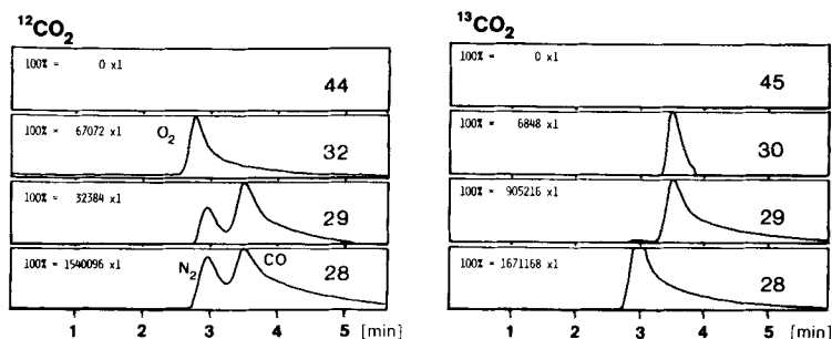
Fig. 2. GC/MS Analysis of photogenerated CO. Gas obtained from photoreduction of ^{12}\text{CO}_2 (left) and ^{13}\text{CO}_2 (right); the mass peaks are recorded at very different sensitivities, indicated by the figure for 100% (= height of strongest peak) at left and decreasing from top to bottom (for example CO at mass 29 on left is natural abundance ^{13}\text{CO} ); abscissa: GC retention time in min.
