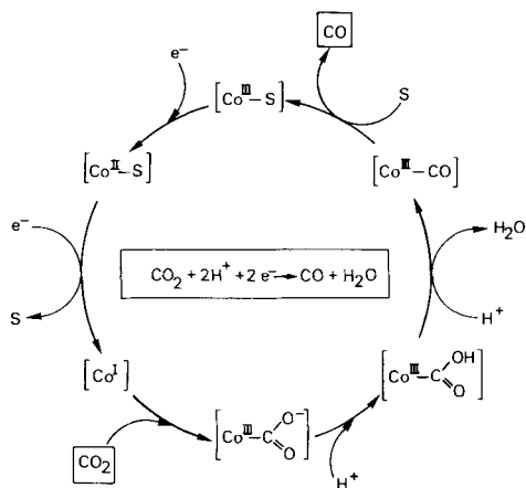
Fig. 10. Schematic representation of a possible catalytic \text{Co} cycle for reduction of \text{CO}_2 to \text{CO} via direct reaction of \text{Co(I)} with \text{CO}_2 to give a \text{Co(III)} -carboxylate intermediate. The electrons are provided by the added electron donor via the photochemical \text{Ru} cycle (Fig. 7); the dielectronic \text{CO}_2 to \text{CO} reduction shown as insert has a potential of -0.52\text{ V} [8] and is, therefore, thermodynamically feasible via \text{Co(I)} complexes (see Text ); \text{S} : solvent or other ligand molecule.
