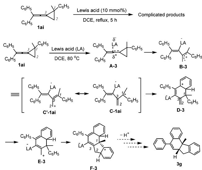
SCHEME 5. Lewis-Acid-Catalyzed Rearrangement of Arylvinylidenecyclopropane 1ai
