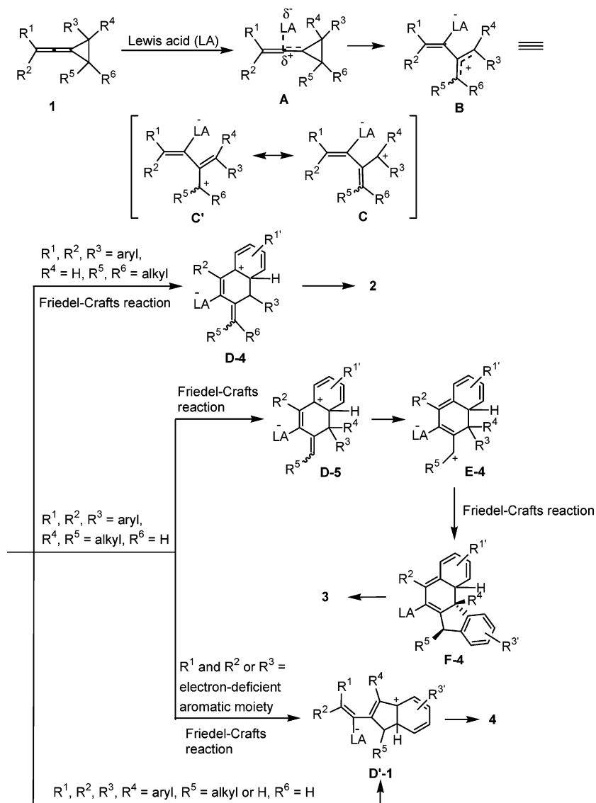
SCHEME 6. Summary of Lewis-Acid-Catalyzed Rearrangement of Arylvinylidenecyclopropanes 1
