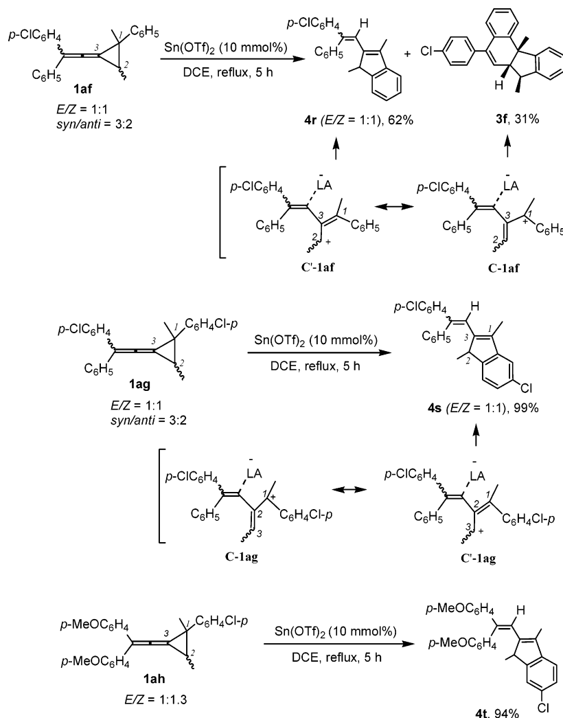
SCHEME 5. Lewis-Acid-Catalyzed Rearrangement of Arylvinylidenecyclopropane 1ai
