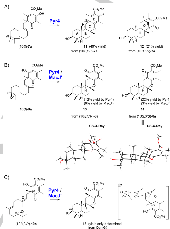
Scheme 1. Structures of isolated meroterpenoids obtained from Pyr4- and MacJ'-mediated reactions with A) (10S)- 7a ; B) (10S)- 8a ; C) (10S,3'R)- 10a .
