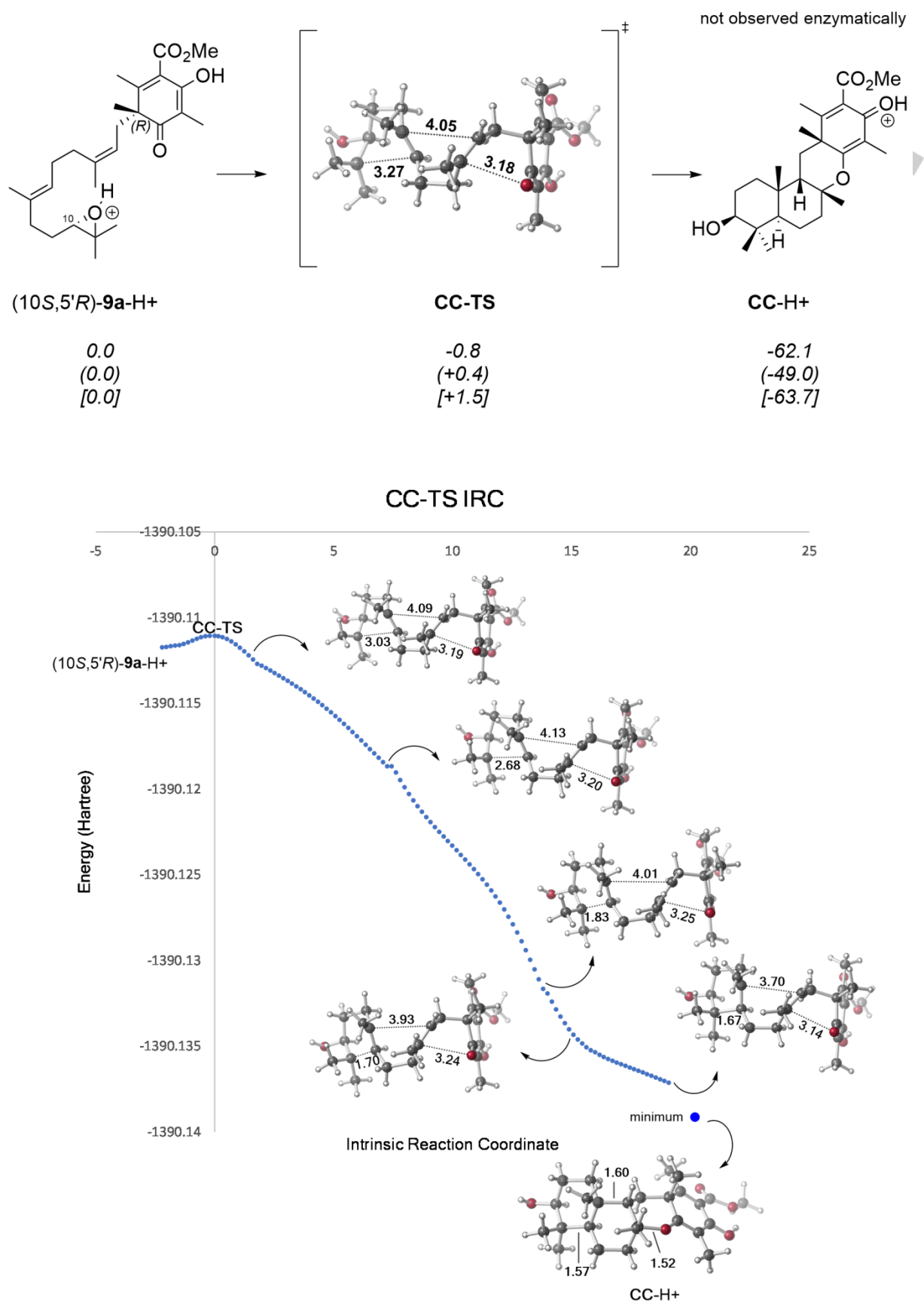
Figure 6. DFT calculations for the cyclization mechanism for the formation of CC . Computed (B3LYP-D3(BJ)/6-31G(d,p)//B3LYP/6-31G(d,p) (on top), CPCM(H 2 O)-B3LYP-D3(BJ)/6-31G(d,p)//B3LYP/6-31G(d,p) (in parentheses) and MPW1PW91/6-31G(d,p)//B3LYP/6-31G(d,p) [in brackets]) relative free energies (kcal/mol, italics) for minima and transition state structures (TSSs) and IRC traces for the respective TSSs. Bond distances are in Angstroms (Å).
