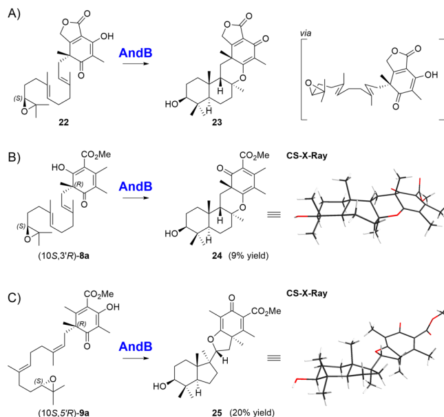
Scheme 3. A) Natural reaction of AndB and structures of isolated meroterpenoids obtained from AndB-mediated reactions with B) (10 S ,3' R )- 8a ; C) (10 S ,5' R )- 9a .
