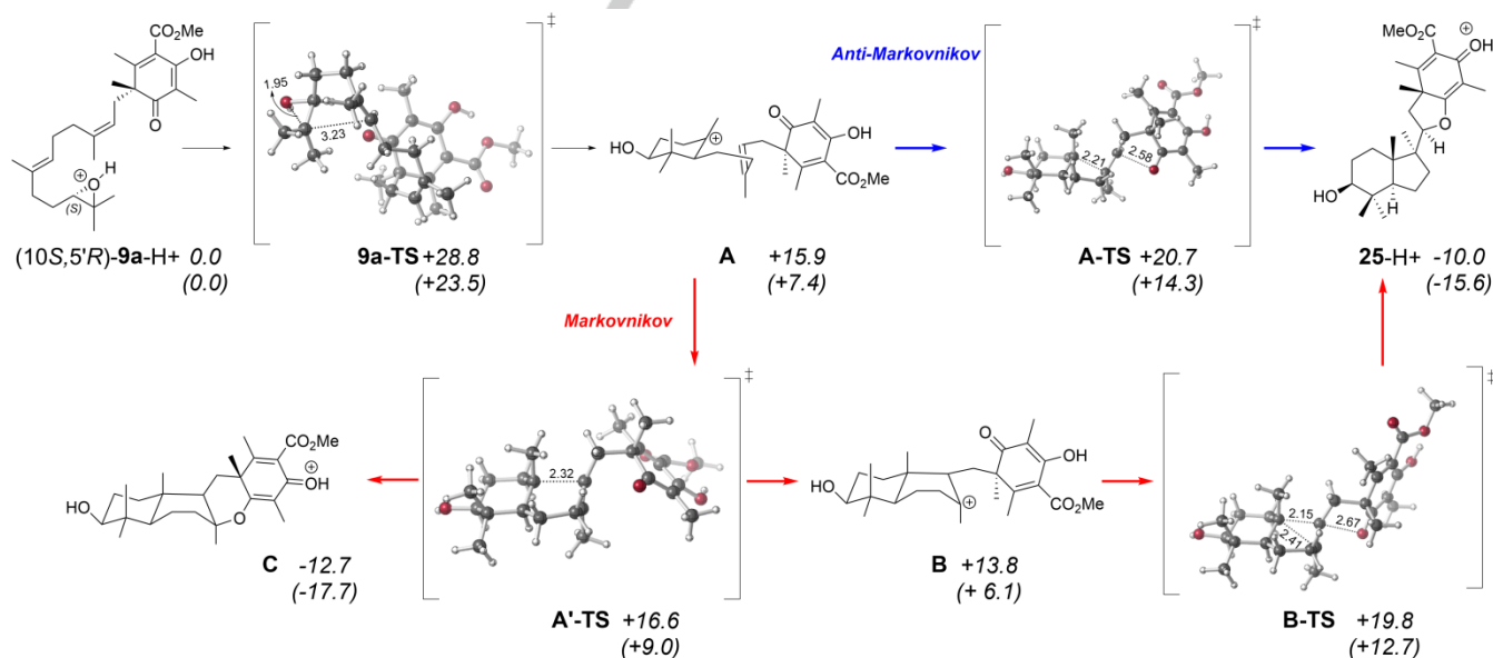
Figure 4. DFT calculations for the cyclization mechanism of (10 S ,5' R )- 9a towards 25 by AndB. Two conformers of A were located, one connected to 9a-TS and another connected to A-TS , which differ in energy by 0-3 kcal/mol, depending on the level of theory; see SI for details. Computed (B3LYP-D3(BJ)/6-31G(d,p)//B3LYP/6-31G(d,p) in black (top), CPCM(H 2 O)-B3LYP-D3(BJ)/6-31G(d,p)//B3LYP/6-31G(d,p) in parentheses (bottom)) relative free energies (kcal/mol, italics ) for minima and transition state structures (TSSs) involved in formation of compound 25 . Bond distances are in Angstroms (Å).
