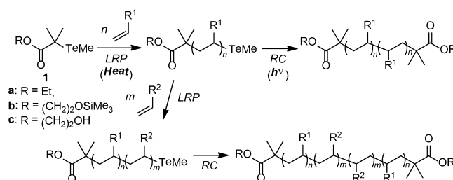
Scheme 1. Sequential LRP-RC, and Its Application to the Synthesis of ABA-Triblock Copolymers
