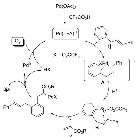
Scheme 2. Proposed Mechanism for the Pd-Catalyzed Olefination Reaction
