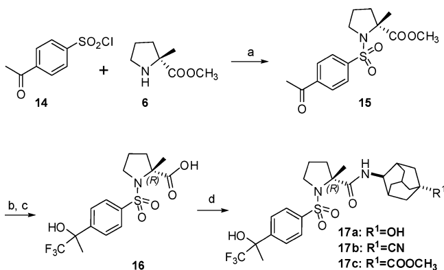
Scheme 3. Synthesis of Compounds 17a–c a
