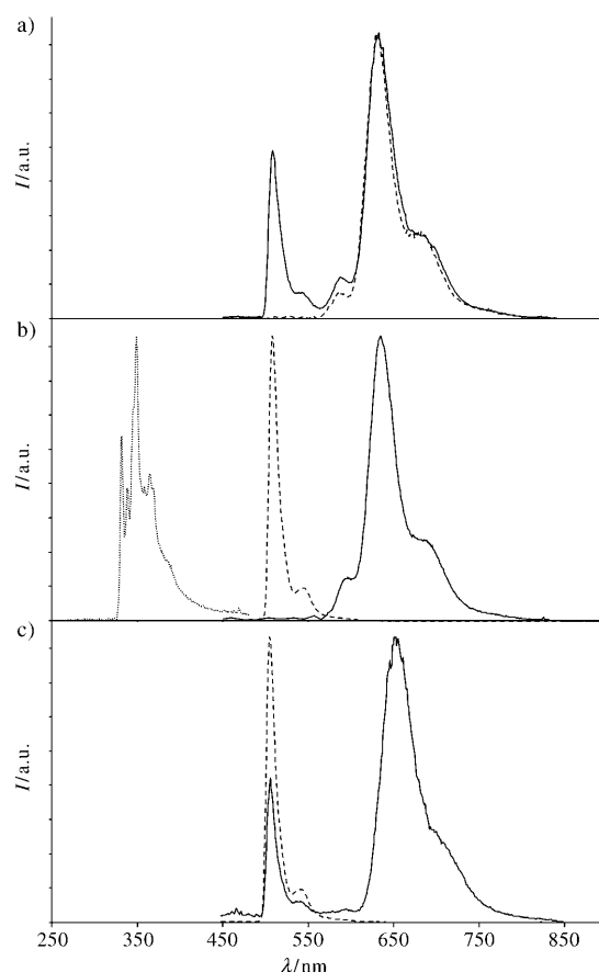
Figure 6. Emission spectra of the studied compounds in a butyronitrile rigid matrix at 77 K. a) 1 (—) and 5 (-----). b) 4 (.....), 6 (-----), and 7 (—). c) 2 (—) and 6 (-----). Compounds 1 and 2 are excited at 480 nm. The spectra of the other species are independent of excitation wavelength.
