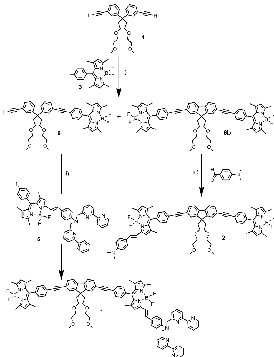
Scheme 1. i) Compound 3 (1 equiv), [Pd(PPh 3 ) 4 ] (10 mol %), C 6 H 6 /Et 3 N, 60 °C, 15 h, 25% of 6b , 21% of 6 ; ii) compound 5 (1 equiv), [Pd(PPh 3 ) 4 ] (10 mol %), C 6 H 6 /Et 3 N, 60 °C, 15 h, 42%; iii) 4-dimethylbenzaldehyde (1 equiv), toluene, piperidine, Dean Stark, trace p -TsOH, 45%.
