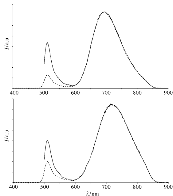
Figure 5. Normalized emission spectra of 1 (top panel) and 2 (bottom) in acetonitrile at room temperature. Excitation is 480 nm (—) or 335/350 nm (----).
