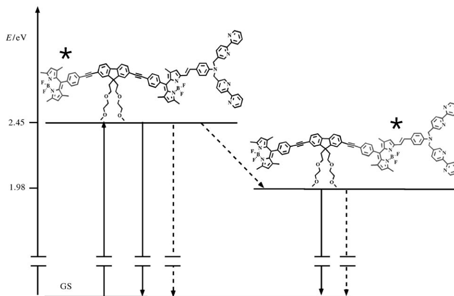
Figure 8. Energy-level diagram schematizing the energy-transfer process in 1 . GS stands for ground state. In the excited states, the asterisk indicates the Bodipy subunit at which the excited-state energy is located. Solid and dashed lines stand for radiative and radiationless transitions, respectively. The excited-state energies are approximated to the 77 K emission maxima (see Table 1) of the two Bodipy subunits.
