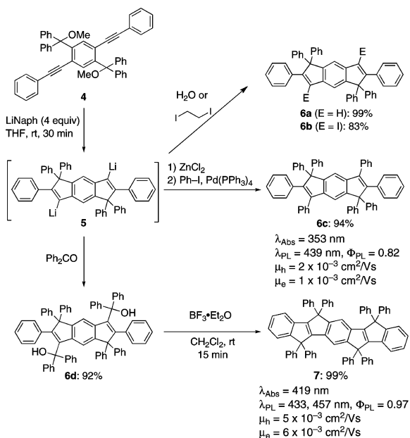
Scheme 2. Modular Synthesis of Dihydro- s -indacenes 6 and Diindenoindacene 7
