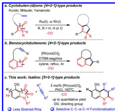
Scheme 1. Decarbonylative C–C Activation of Cyclic Ketones with Insertion of an Unsaturated Moiety
