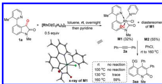
Scheme 3. Mechanistic Exploration
