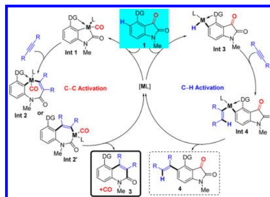
Scheme 2. Reaction Pathways: C–C vs C–H Activation
