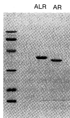
Fig. 2. SDS-Polyacrylamide Gel Electrophoresis of the Purified Aldose Reductase and Aldehyde Reductase from the Medulla of Rat Kidney
