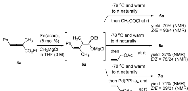
Scheme 3. Mechanistic Study
