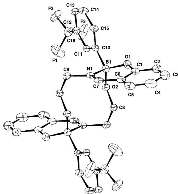
Fig. 4. Molecular structure of compound 17i .
