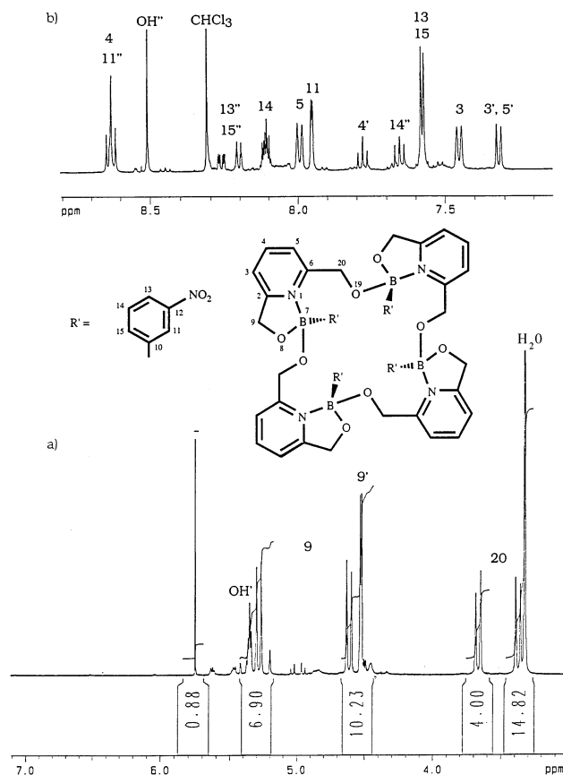
Fig. 2. ^1\text{H} -NMR spectrum of compound 16 in \text{DMSO}-d_6 : (a) aliphatic region; (b) aromatic region. The signals of the starting materials are marked with ' for the 2,6-pyridinedimethanol and '' for the 3-nitrophenylboronic acid. The signal of \text{H}_2\text{O} results from an impurity in \text{DMSO}-d_6 . \text{CHCl}_3 is forming part of the crystal lattice of compound 16 .
