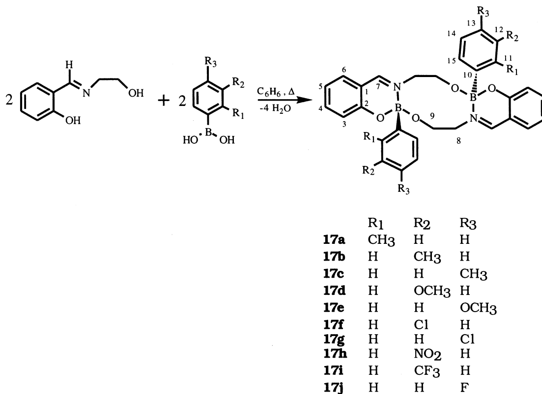
Scheme 2. Preparation of compounds 17a–j .
