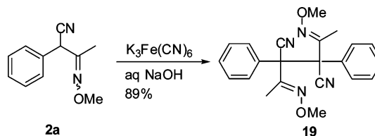
SCHEME 2. An Oxidative Coupling Reaction of 2a Mediated by \text{K}_3\text{Fe}(\text{CN})_6
