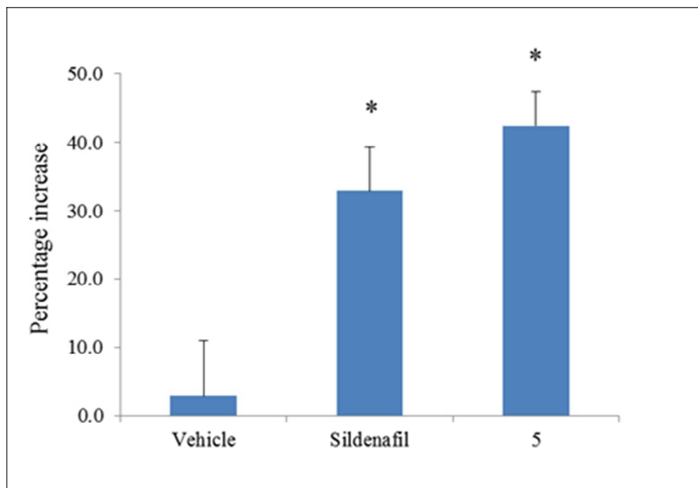
Effect of compound 5 on ICP/BP 30 min after p.o. administration (10 mg/kg) in the rat erection model. Data are expressed as Mean \pm SD (n=3). Percentage increase: ((ICP/BP)after-(ICP/BP)before) / ((ICP/BP)before100%, *: compared with vehicle P < 0.05 , student's t-test. 84x58mm (150 x 150 DPI)
