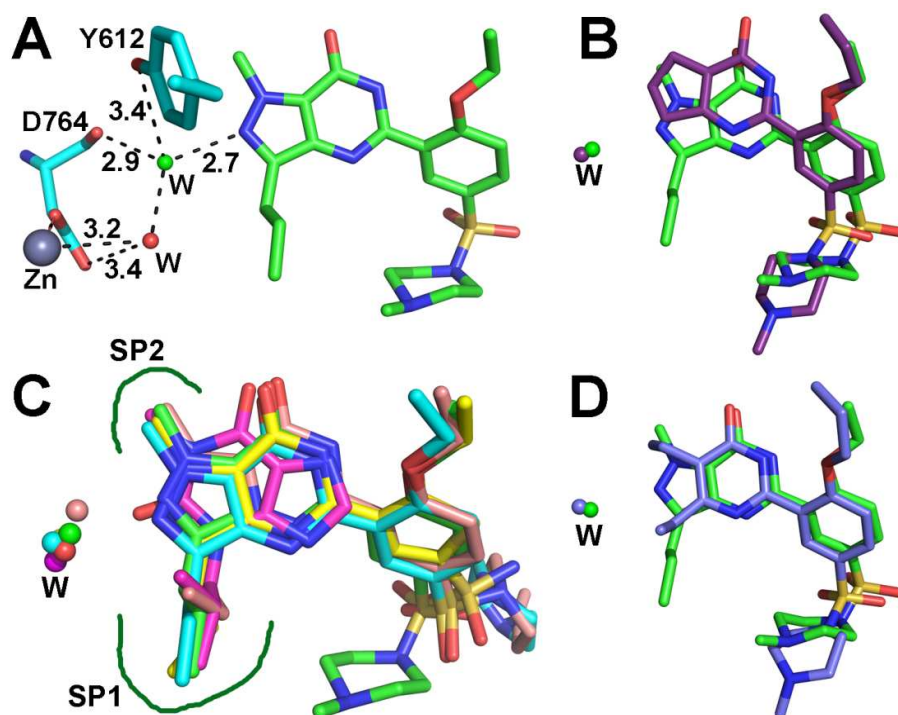
Figure 1. A crucial water molecule in the crystal structures of PDE5 in complex with different inhibitors. The complex structures were superimposed by fitting all the C \alpha atoms of the enzyme. (A) The H-bond interactions of the water molecule with sildenafil, side-chain residues, and the other water molecule in the complex structure of PDE5/sildenafil (pdb code 2H42). (B) Superimposition of compound 2 and sildenafil as well as the crucial water molecule. (C) Superimposition of inhibitors in five complex structures with pdb codes 1UDT (cyan), 2H42 (green), 1RKP (magenta), 3BJC (yellow), and 3B2R (wheat). The water molecules at the same location in these five complex structures as well as in the apo structure (pdb code 2H40, red) are shown as colored balls. SP1 and SP2 represent two sub-pockets that interact with substituents of the
