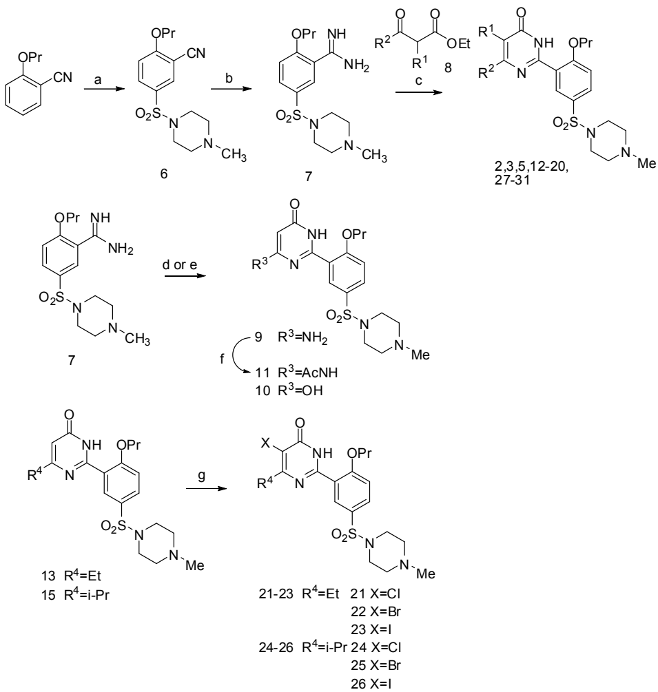
Scheme 2. The synthesis of compounds with monocyclic pyrimidinone core
