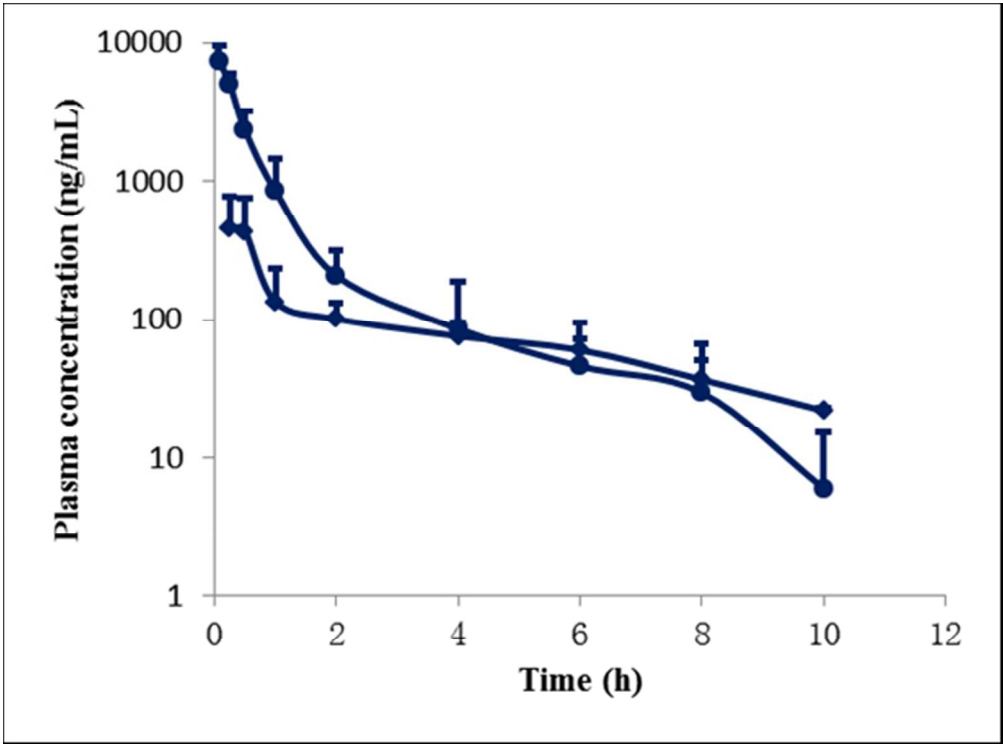
Mean plasma concentrations of compound 5 in male rat, after single p.o. 10 mg/kg (◆) & i.v 5 mg/kg (●). Data used to generate the profile are the Mean±SD from three male rats (individual samples at all time points). 174x129mm (89 x 89 DPI)
