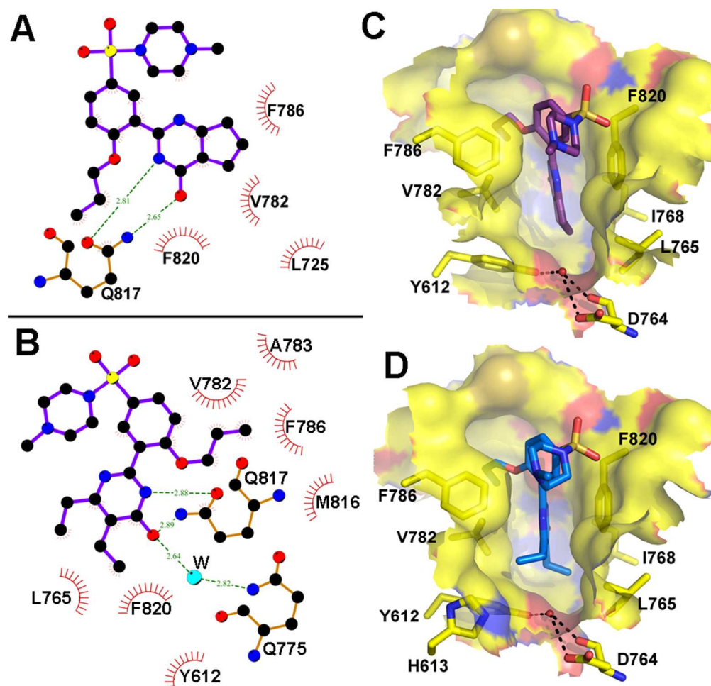
The interactions between two compounds (2 and 5) and PDE5 in crystal structures of their complexes. (A, B) LIGPLOT representations of the interactions of compounds 2 (A) and 5 (B) with the enzyme. (C, D) Molecular surface of the binding pockets for compounds 2 (C) and 5 (D) in their complex structures with the PDE5 catalytic domain. The crucial water molecule is shown as a red ball and the H-bonds formed between it and the residues are labeled with black dash lines.
