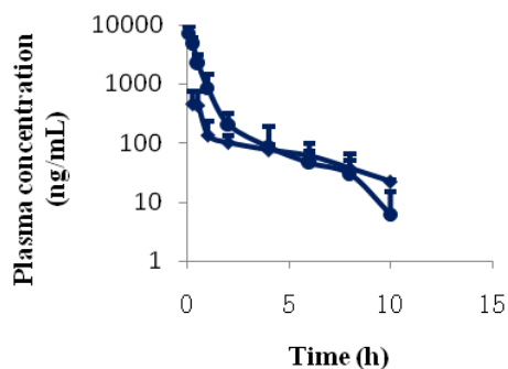
Figure 3. Mean plasma concentrations of compound 5 in male rat, after single p.o. 10 mg/kg (◆) & i.v 5 mg/kg (●). Data used to generate the profile are the Mean±SD from three male rats (individual samples at all time points).
