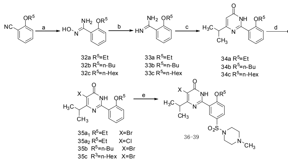
Scheme 3. The synthesis of compounds 36-39
