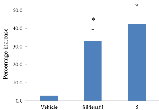
Figure 4. Effect of compound 5 on ICP/BP 30 min after p.o. administration (10 mg/kg) in the rat erection model. Data are expressed as Mean ± SD (n=3). Percentage increase: \frac{(\text{ICP/BP})_{\text{after}} - (\text{ICP/BP})_{\text{before}}}{(\text{ICP/BP})_{\text{before}}} \times 100\% , *: compared with vehicle P < 0.05 , student's t-test.
